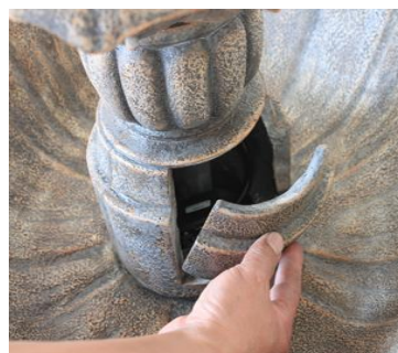
Connect the tubing to the pump then place the pump inside the riser. Install the pump access door.
