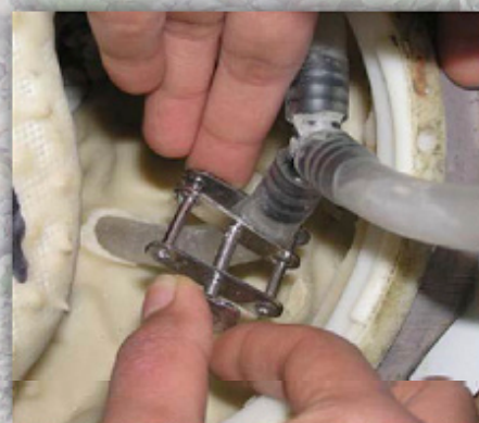
Note restrictor position in top unit, allowing you to fine tune the flow amount
