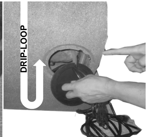
IMPORTANT: to prevent water loss, create a drip-loop with the light cords by dipping them into the reservoir before they exit out the back of the fountain.
